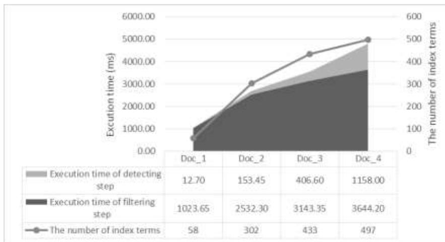
Figure 2: Execution Time Constitution in Plagiarism Detection System
