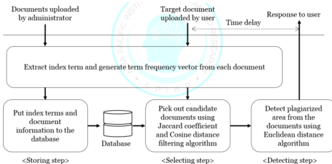
Figure 1: Process Flow of Plagiarism Detection System
