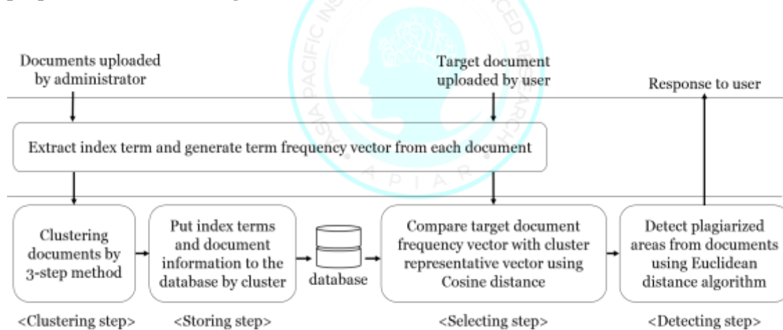
Figure 3: Process Flow of Enhanced Plagiarism Detection System
