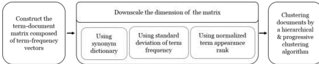
Figure 4: Process Flow of Document Clustering
