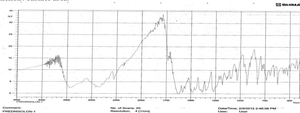
Fig1: FTIR spectra of Prednisolone
