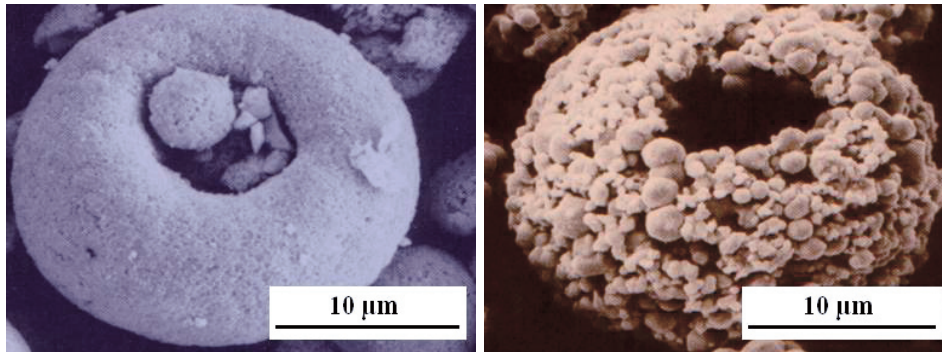
Figure 5 – (SEM) micrography of the \text{Al}_2\text{O}_3 13% \text{TiO}_2 and Mo powder particles Slika 5 – (SEM) mikrografija čestice praha \text{Al}_2\text{O}_3 13% \text{TiO}_2 i Mo Рис. 5 – (SEM) микрография частиц порошка \text{Al}_2\text{O}_3 13% \text{TiO}_2 i Mo
