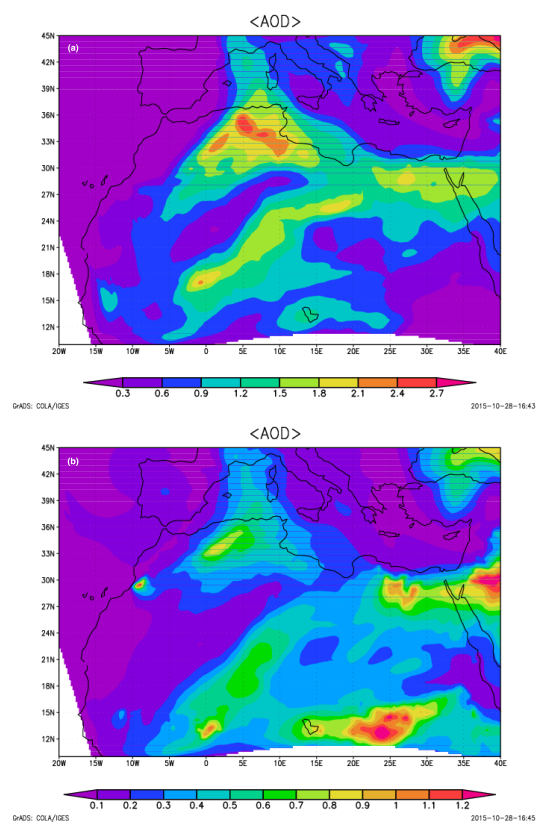
Figure 3: Time Averaged Map of Aerosol Optical Depth 550 nm from WRF-Chem simulation: (a) AFWA dust emission model; (b) S01 dust emission model
