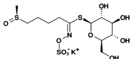
Glucoraphanin
