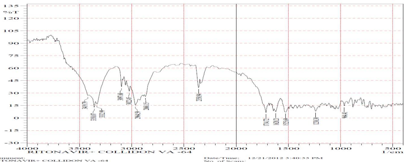
Fig. 5: FT-IR spectra for Ritonavir and Kollidon VA64 (Physical mixture)
