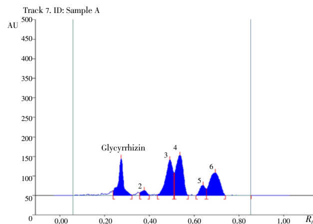
Figure 3. HPTLC chromatogram of GGRMe scanned at 254 nm. Mobile phase–Ethyl acetate: glacial acetic acid: methanol: water (4:3:1:0.5, v/v/v/v).
