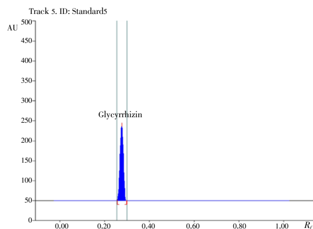
Figure 2. HPTLC chromatogram of standard glycyrrhizin scanned at 254 nm. Mobile phase–Ethyl acetate: glacial acetic acid: methanol: water (4:3:1:0.5, v/v/v/v).
