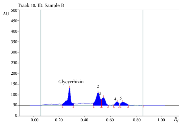
Figure 4. HPTLC chromatogram of LRCMe scanned at 254 nm. Mobile phase–Ethyl acetate: glacial acetic acid: methanol: water (4:3:1:0.5, v/v/v/v).
