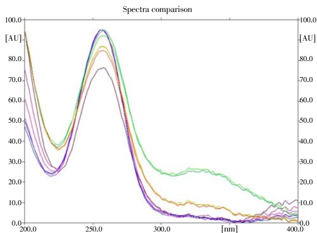
Figure 5. Spectral comparison of glycyrrhizin and different samples.
