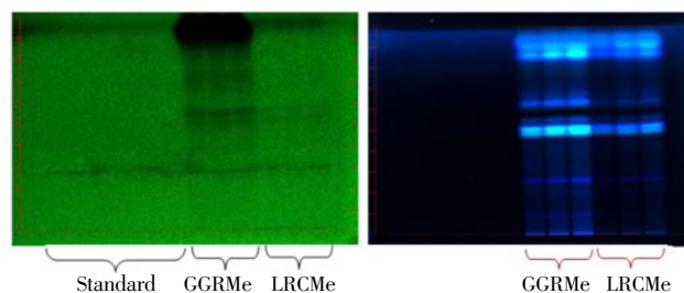
Figure 1. Picture of developed HPTLC plate at 254 nm and 366 nm.
