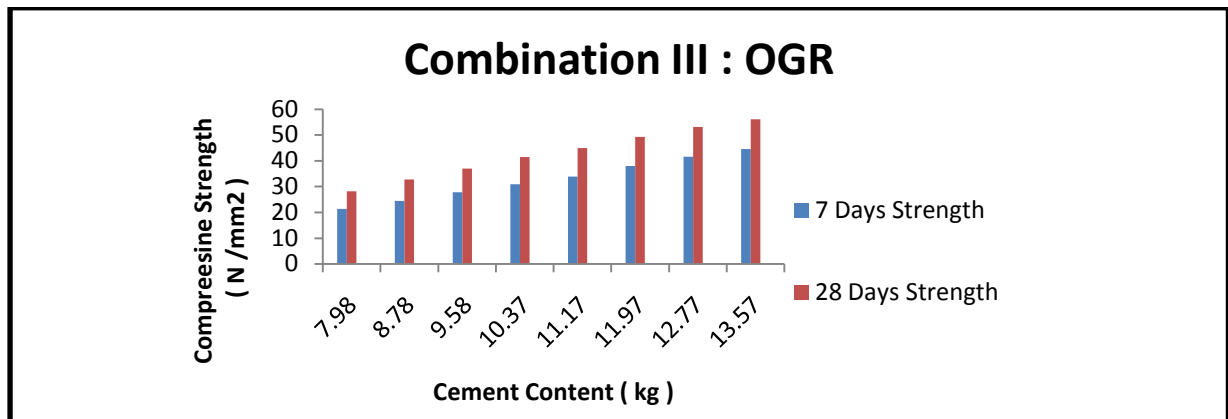
Fig. 1.(Variation in compressive strength with cement content)
