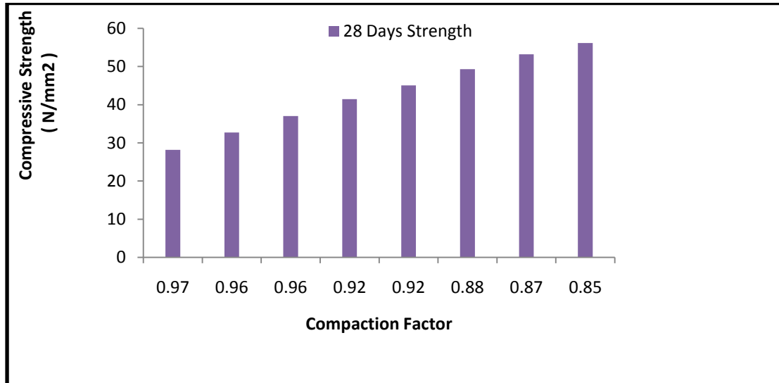
Fig. 2. (Variation in compressive strength with compaction factor)
