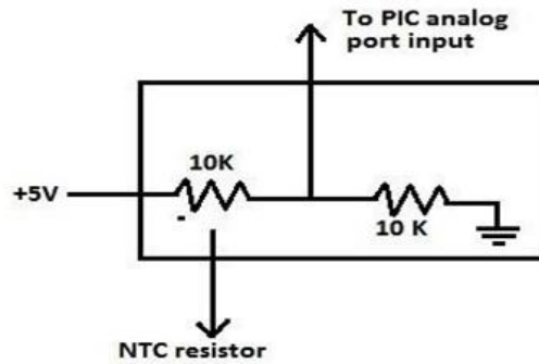
Figure.4. Temperature Sensor
