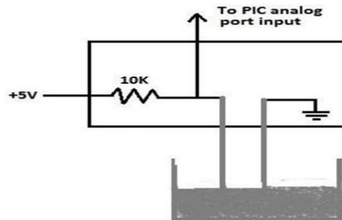
Figure 5: Drip Sensor
