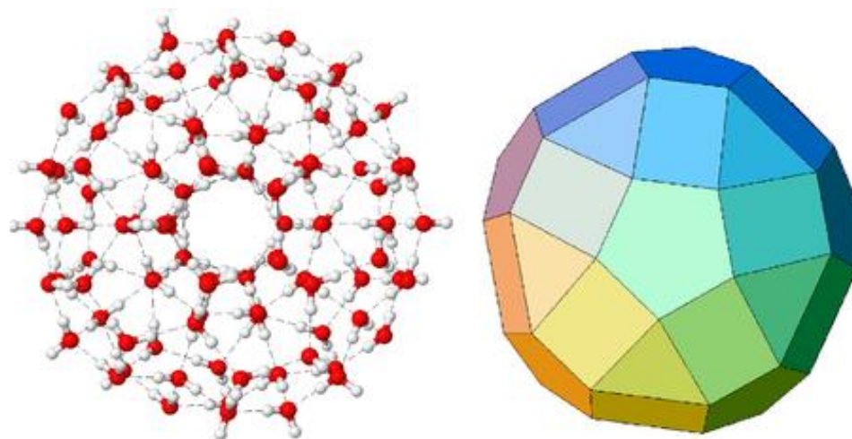
Figure 12: Icosahedron cluster based on 100 \text{H}_2\text{O} molecules and the underlying structure according to M. Chaplin’s model
