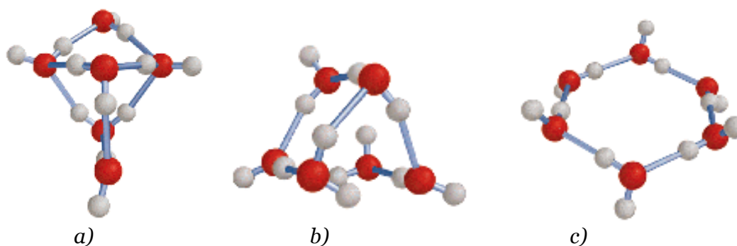
Figure 8: Calculation of small water cluster structures (a–c) with general formula (\text{H}_2\text{O})_n , where n = 6 [29] (Tsai & Jordan, 1993)
