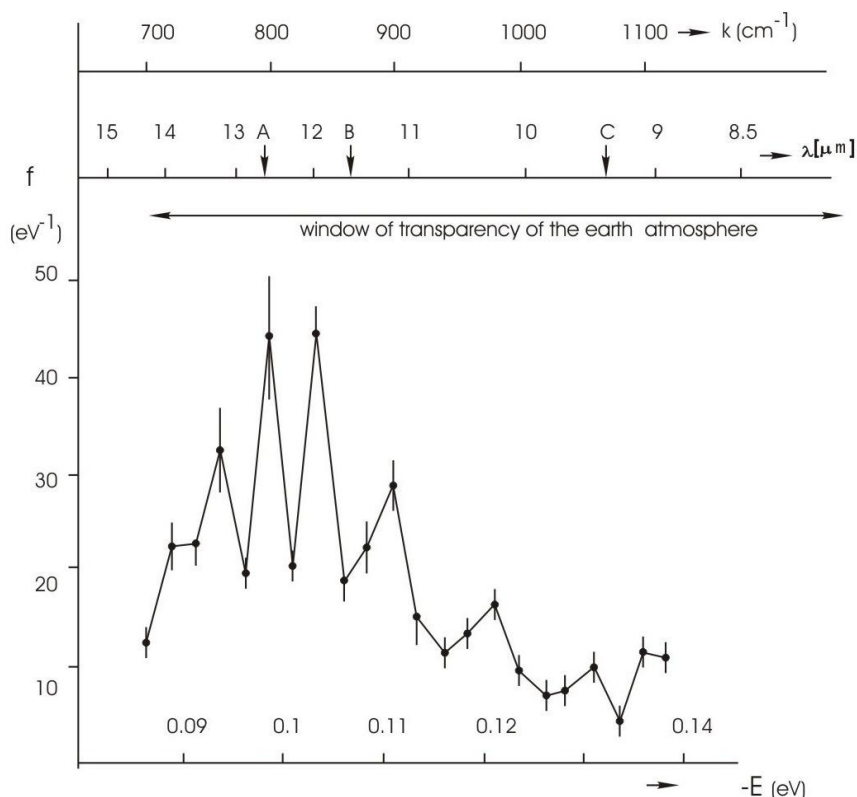
Figure 7: DNES-spectrum of deionized water (chemical purity – 99,99%, pH – 6,5–7,5, total mineralization – 200 mg/l, electric conductivity – 10 \mu\text{S}/\text{cm} ). On the horizontal axis shows the energy of the H...O hydrogen bonds in the associates – E (eV). The vertical axis – energy distribution function – f ( \text{eV}^{-1} ). k – the wave number ( \text{cm}^{-1} ); \lambda – wavelength (mm)
