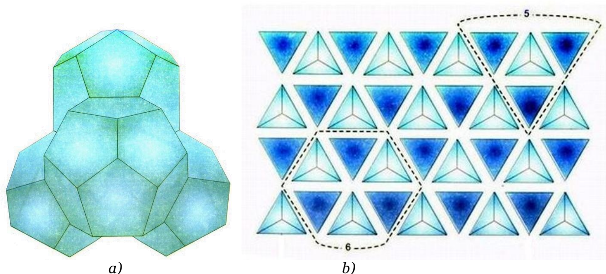
Figure 11: Model of water associate according to the model of S.V. Zenin [33]: a ) – associate of 57 \text{H}_2\text{O} molecules, tetrahedron of four dodecahedron (“quantum”); b ) – bulk packaging of “quanta”
