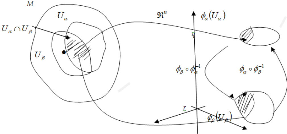
Figure 1: The smooth maps \phi_\alpha \circ \phi_\beta^{-1} on the n -dimensional Euclidean space \mathbb{R}^n giving the change of coordinates in the overlap region.
