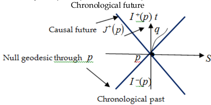
Figure 3: Causality and chronology in M .
