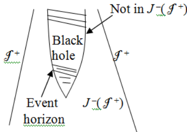
Figure 4: The black hole is a region of space-time from which no causal communications, that is, non-spacelike curves can reach the future null infinity I^+ .
