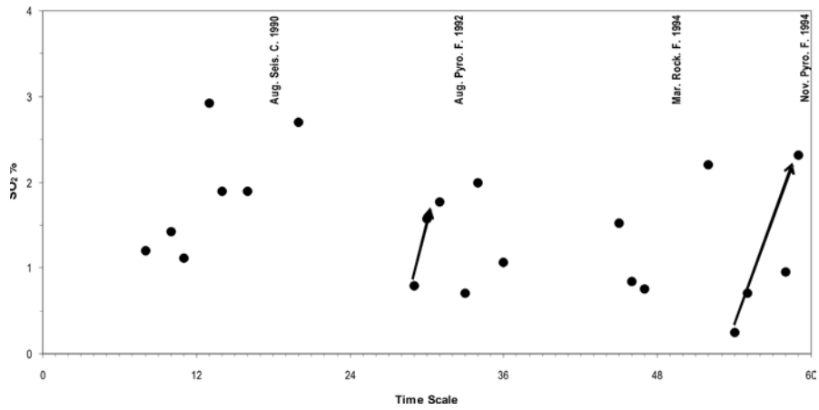
Figure 9. SO 2 , Gendol Merapi Volcano.
