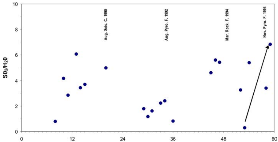
Figure 11. SO 2 /H 2 S, Gendol Merapi Volcano.
