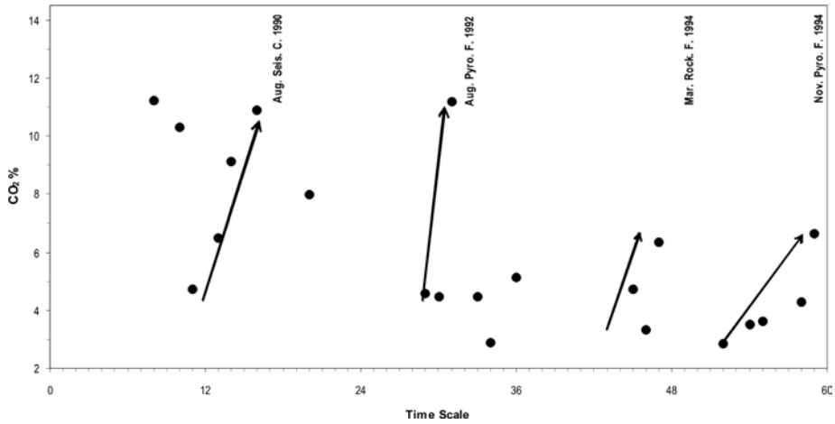
Figure 10 . CO 2 , Gendol Merapi Volcano.
