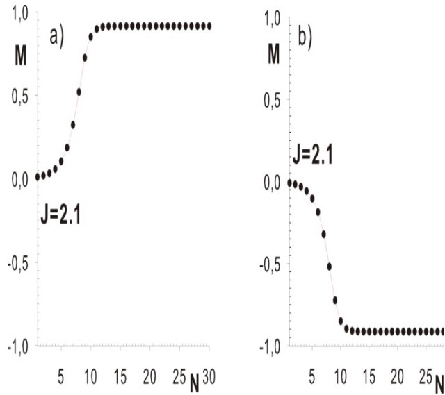
Figure 3. Orbit of the map given by Eq. (1a'): a) initiating from +0.001 and b) initiating from -0.001. Parameters values are \beta^{-1} = 0.5 eV, D = 2.2 eV, J = +2.1 eV. Orbits initiating from any point in the interval (-1, 0) yield the fixed point -1. Orbits initiating from any point in the interval (0, +1) yield the fixed point +1. Since attraction domains of the fixed points \pm 1 are different, these points do not form a 2-cycle.
