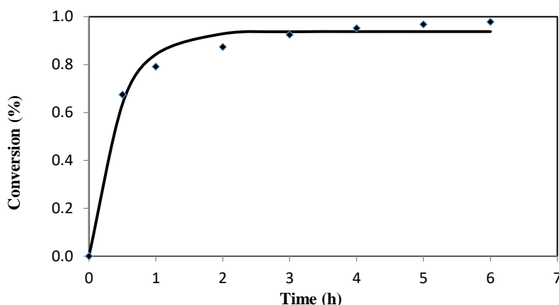
Figure 2: Effect of rate of reaction on hydrolysis of flax seed methyl ester.(Reaction temperature 60oC, enzyme concentration 4%, buffer to flax seed methyl ester ratio of 1.5:1(v/w)) ◆ experimental values — model values
