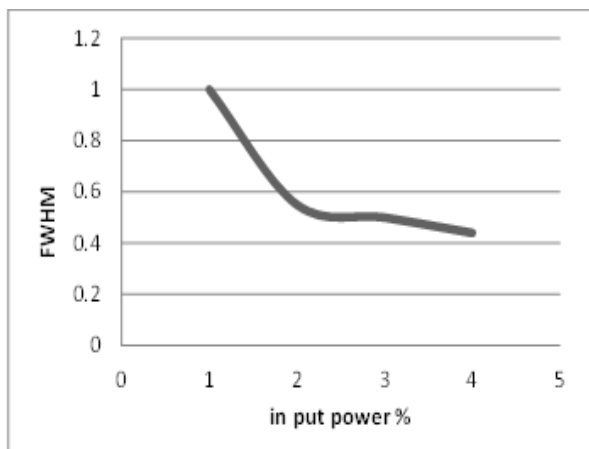
Figure(5)shows the FWHM as a function of input power of OPF doped RB
