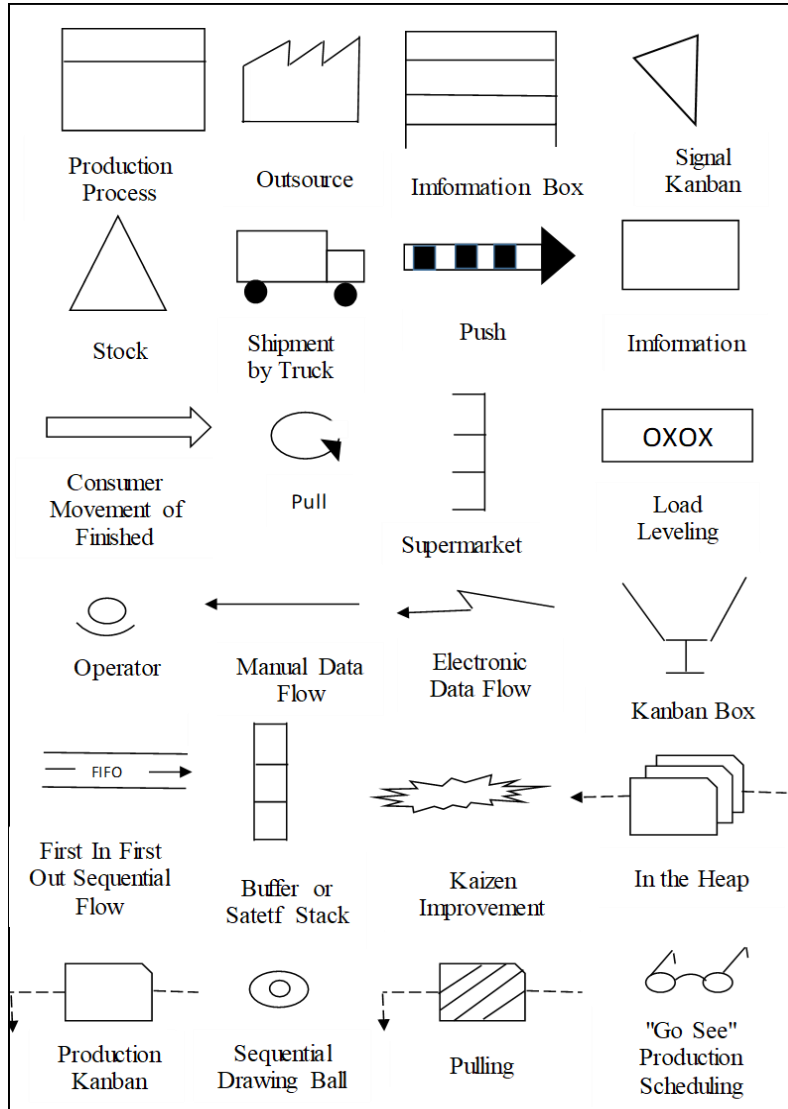
Figure 1. Symbols Used in Value Stream Mapping (from [2])
