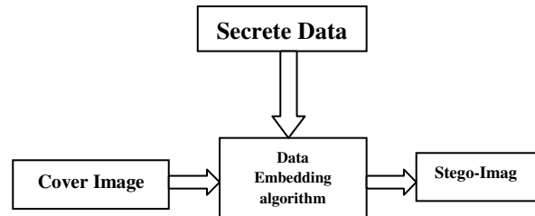
Fig 1: Steganography Diagram
