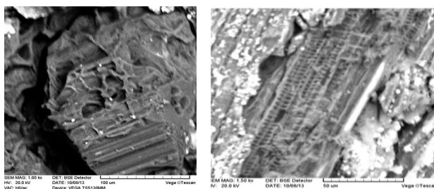
Figure 1. SEM image of charcoal (Left) prepared from saffron leaves without activating and activated carbon (Right).
