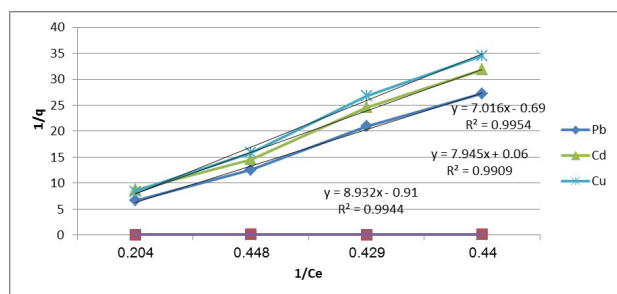
Figure 2. Langmuir adsorption isotherm of copper, cadmium, and lead
