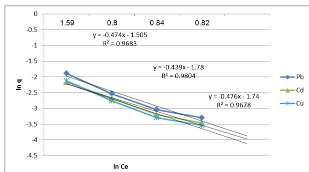
Figure 3. Freundlich adsorption isotherm of copper, cadmium, and lead
